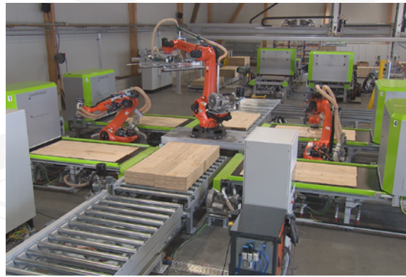
Fully automatic cleaning and repair of panels
